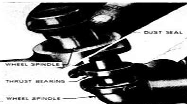
Fig. 2—Top view shows proper installation of dust seal on spindle after spindle is installed in axle extension. Lower view shows proper installation of thrust bearing on spindle prior to installing spindle in axle extension.
