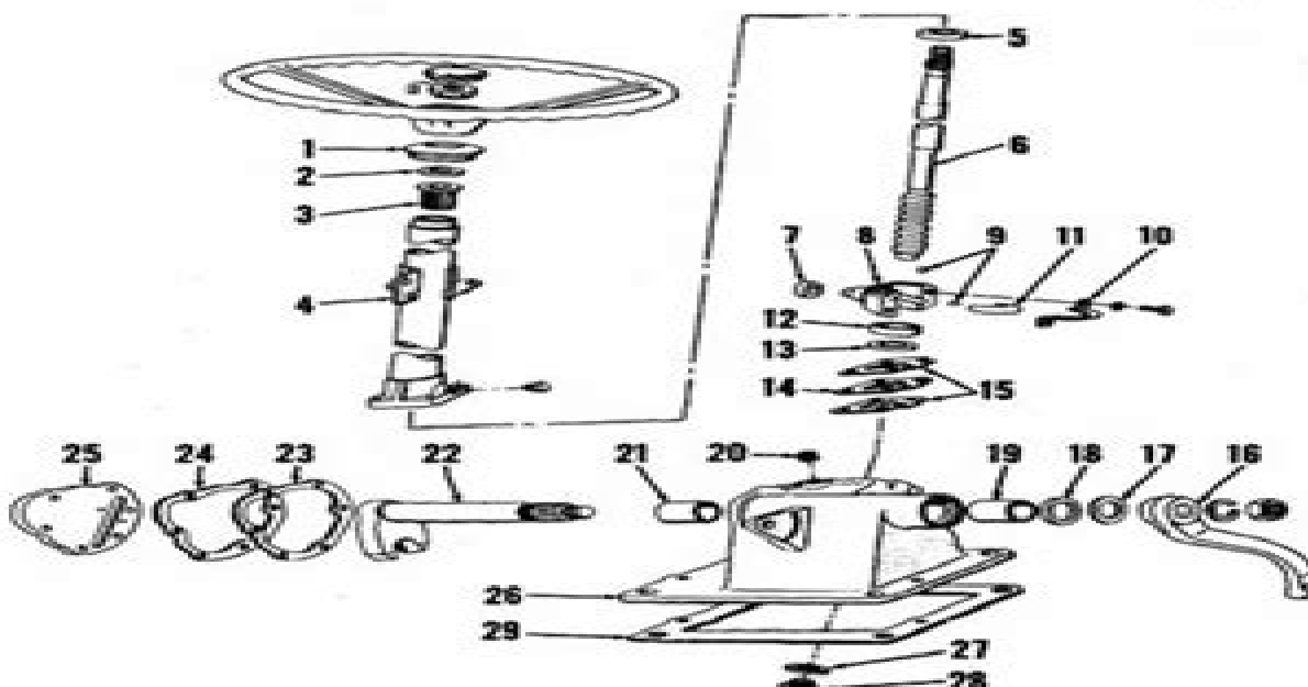
Fig. 3—Exploded view of steering gear unit of the type used on all manual steering models and on early 5100 models with power steering. Thirty-four 1/4-inch (6.35 mm) diameter steel balls are used in the assembly; 20 are used for steering shaft bearings and 14 are used in the ball nut (8) and tube (11) recirculating groove. Parts 27, 28 and 29 are not used on Models 5600, 5610, 6600, 6610, 7600 and 7610.
