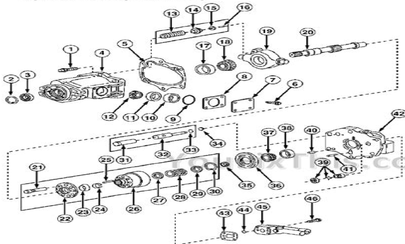
Hydraulic Pump Exploded View
