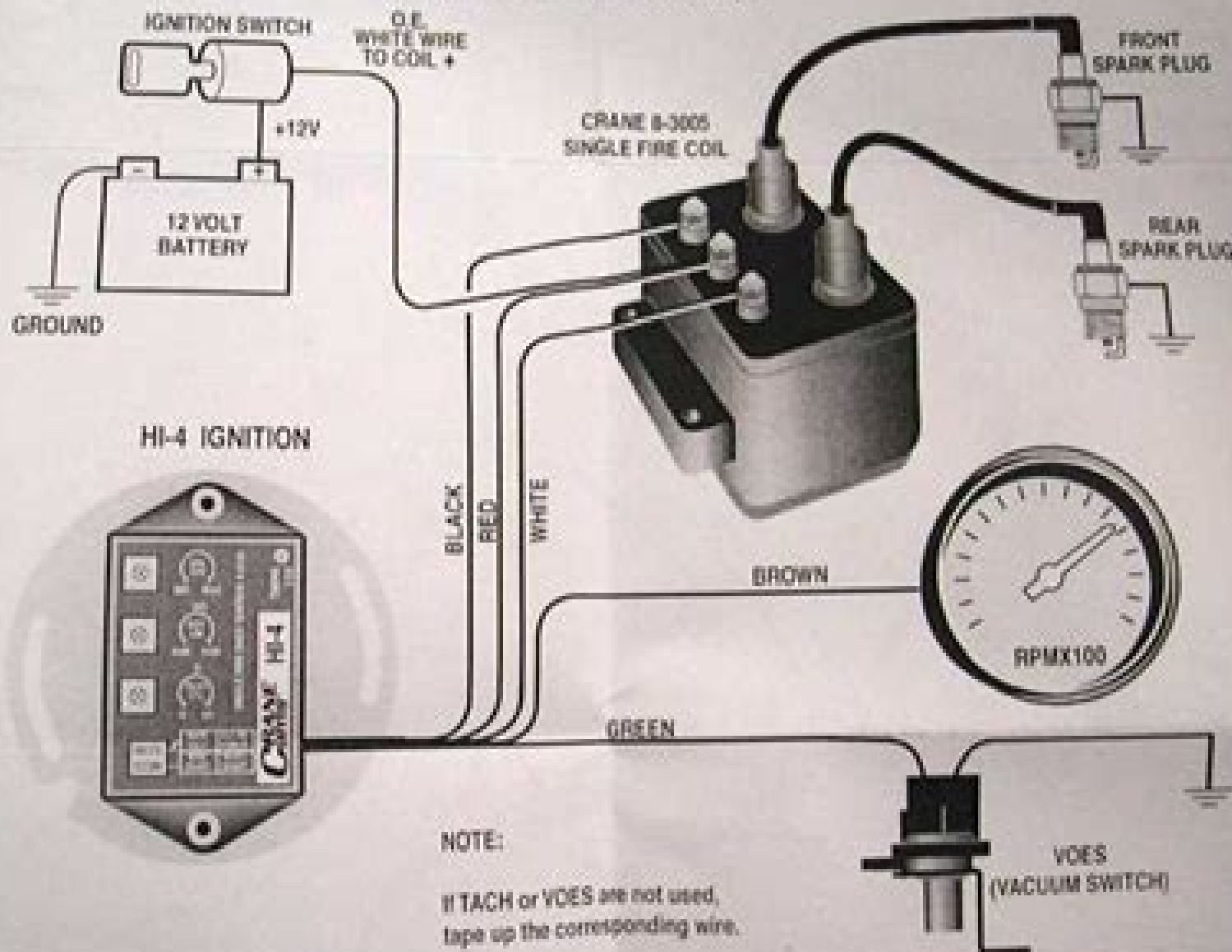
Figure 1. HI-4 Hookup
