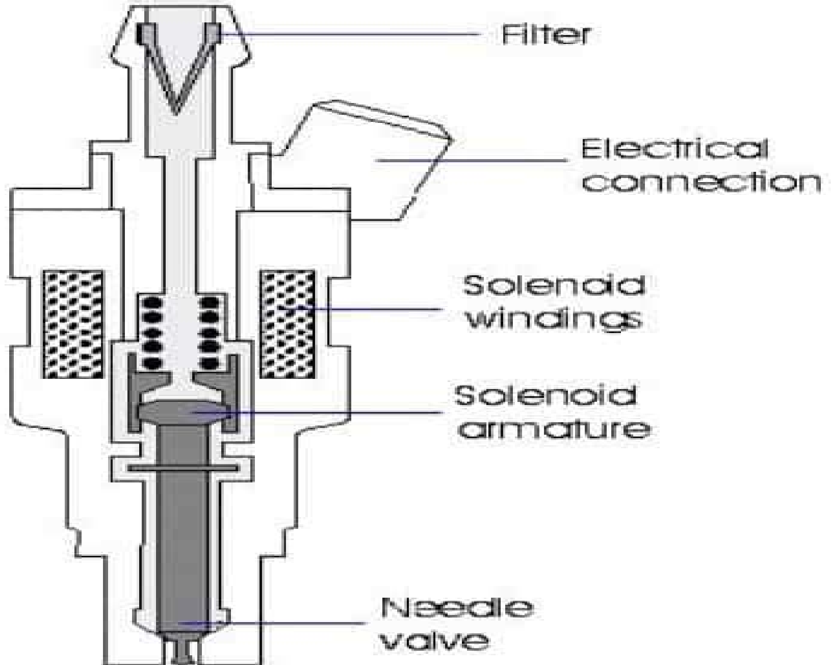
Fig. Electronic Fuel Injector
