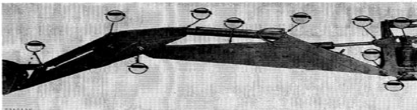
Fig. 62-Backhoe Grease Fittings (12 Points)
