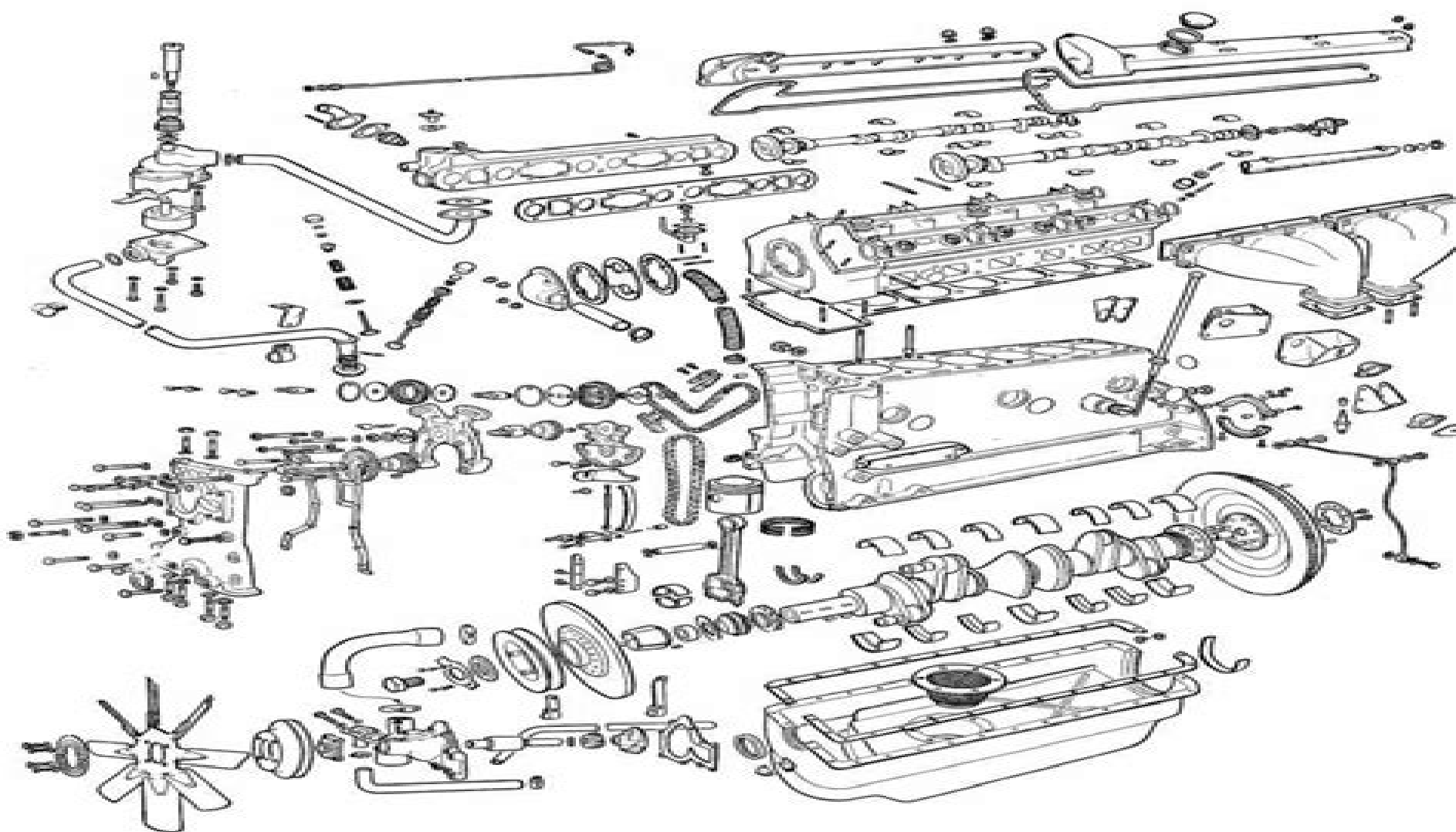
Parts of the engine showing cylinder block, head and sump, crankshaft, con rod and piston assembly, camshafts, camshaft drive sprockets and casing, oil pump, water pump, fan and manifolds
