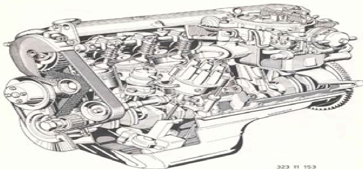
Sectional view of carburetor engine
