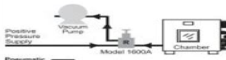
Figure 3. Chamber Purge with Positive Pressure
