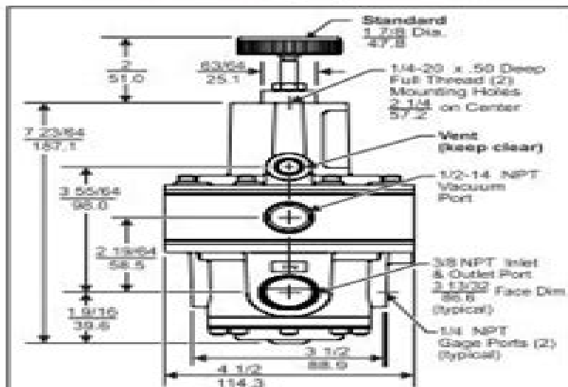
Figure 1. Model 1600A Outline Dimensions
