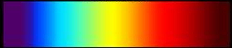
Spectre continu
