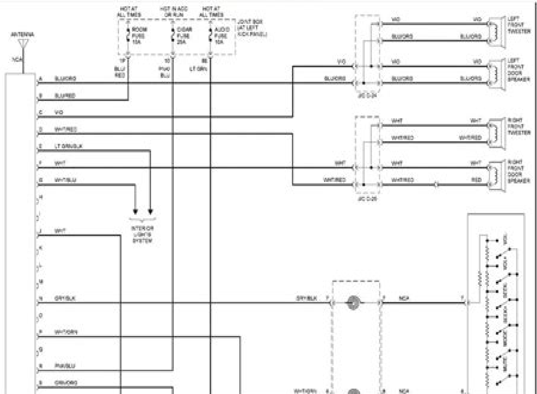
Fig. 32: Radio Circuit
