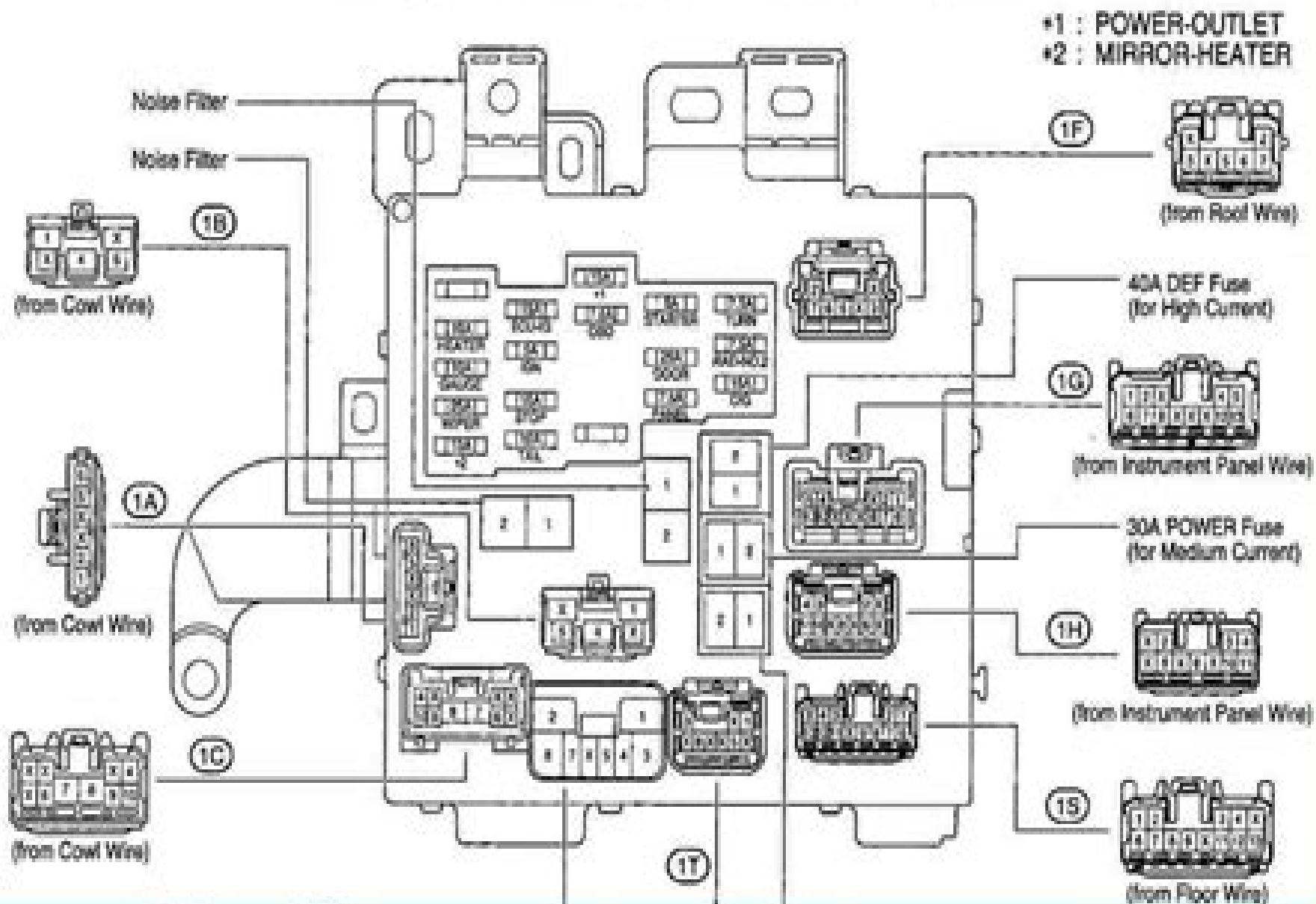
Fig. 2: Identifying Instrument Panel J/B Components Courtesy of TOYOTA MOTOR SALES, U.S.A., INC.
