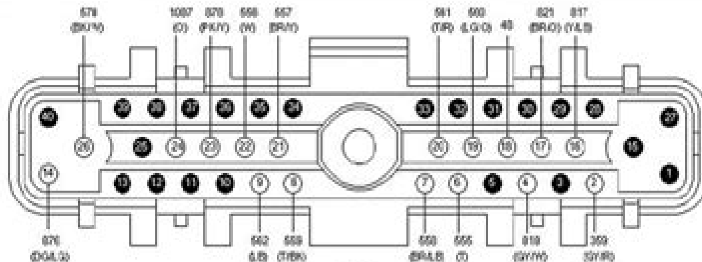
G298 INJECTOR DRIVER MODULE (IDM)
