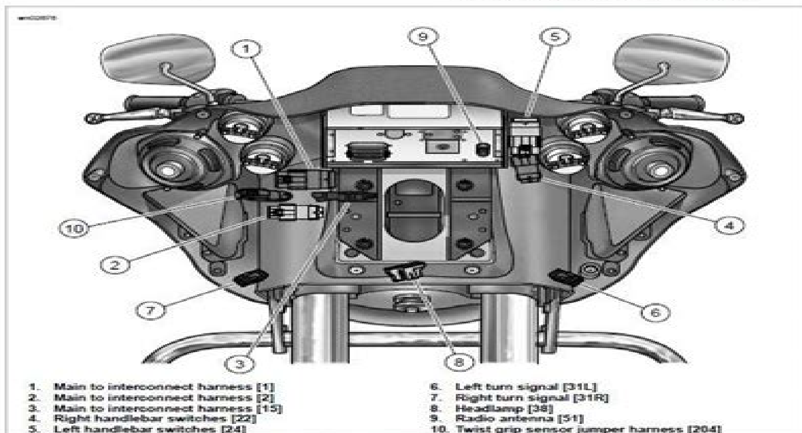
Figure 2-152. Inner Fairing Connectors (FLTR)
