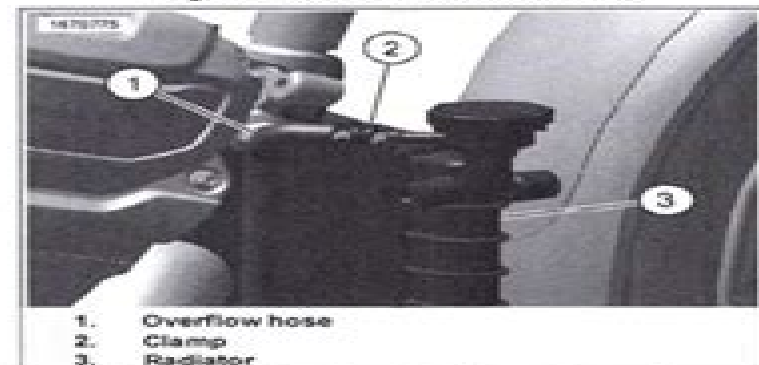
Figure 7-14. Upper Overflow Hose Connection
