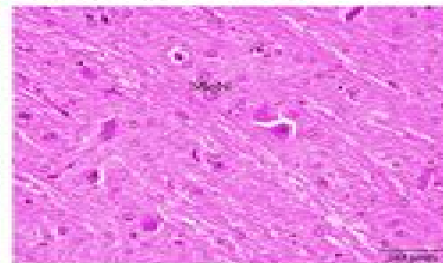
Medulla oblongata
