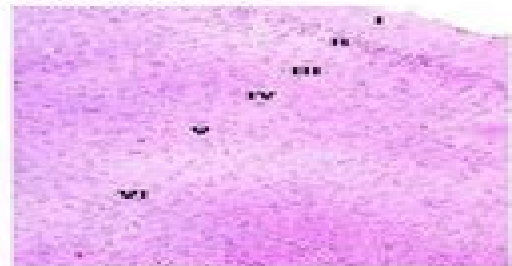
Cerebral cortex
