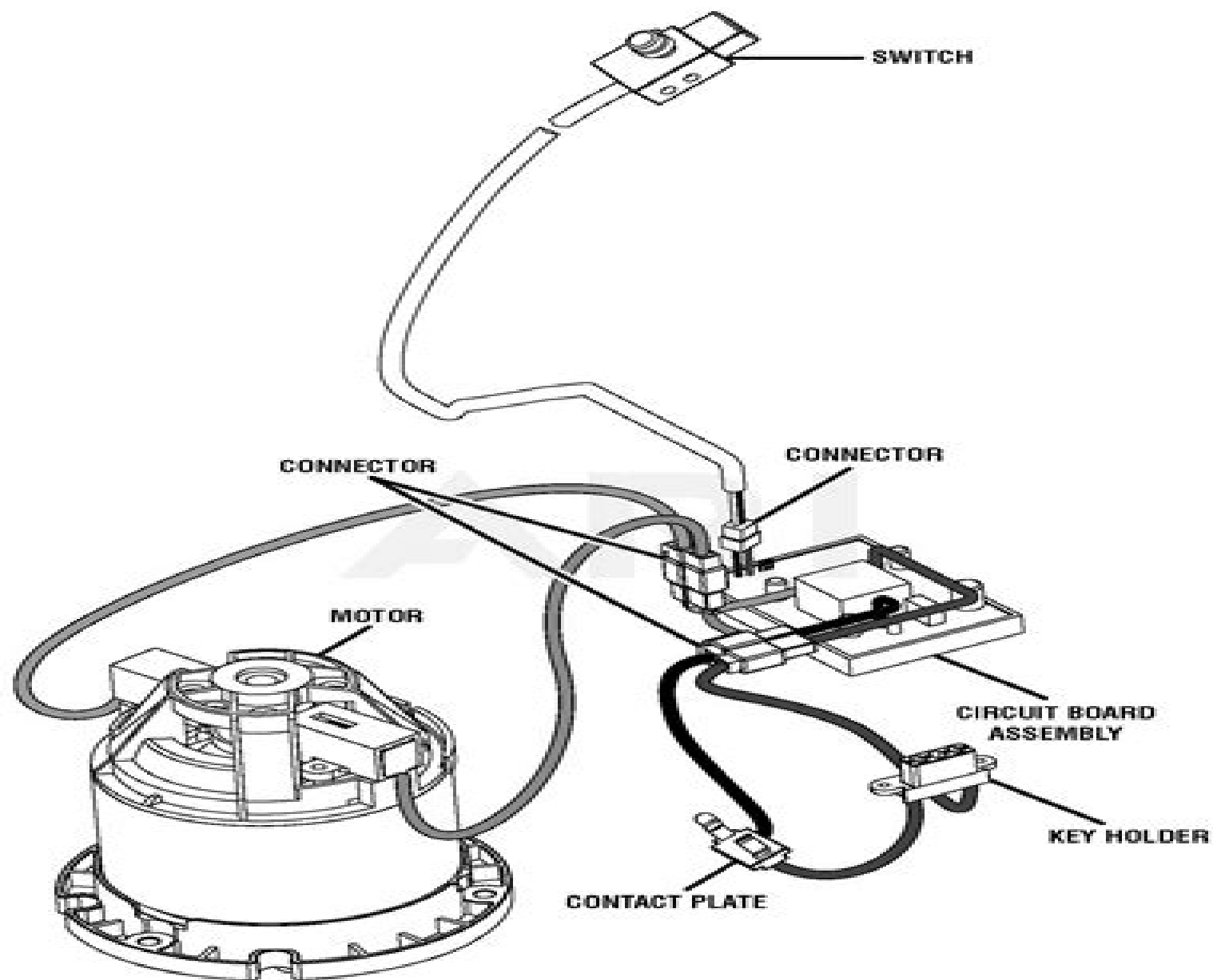
WIRING DIAGRAM
