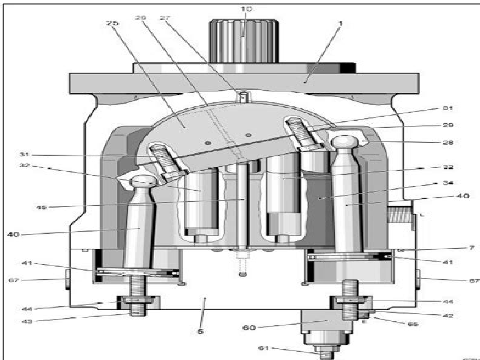
Fig.3 Sectional view Var. displ. motor
