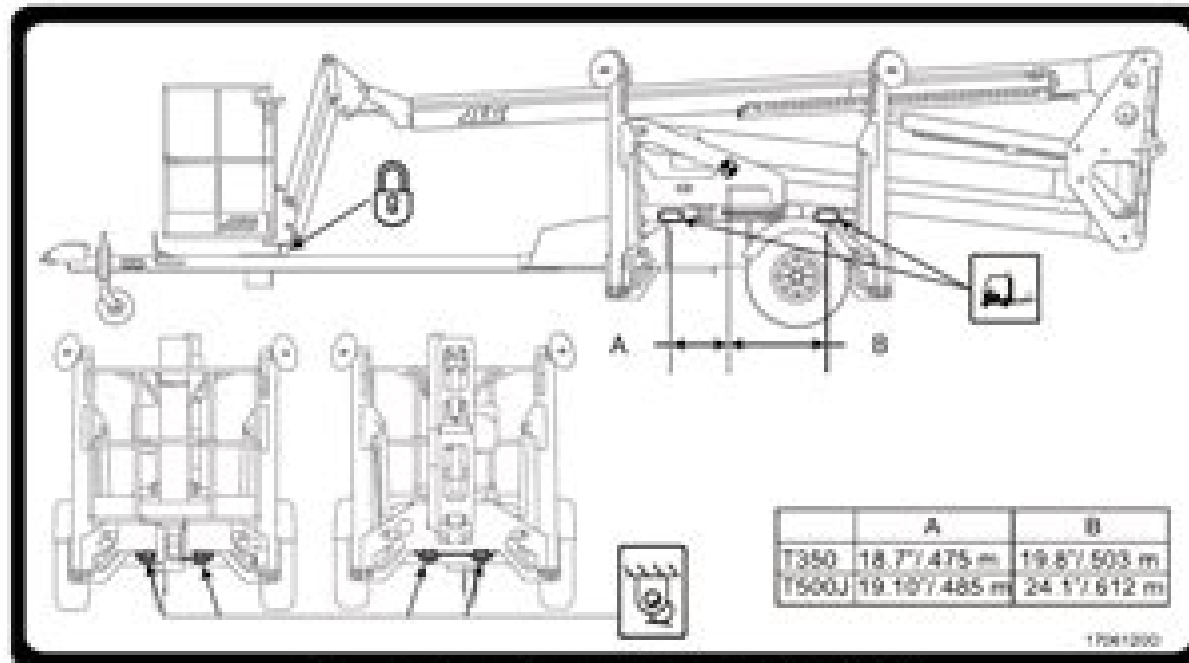
Figure 5-8. Lifting and Tie Down Chart Prior to S/N 6030000864
