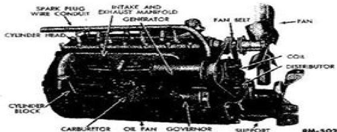
Fig. 2—Right \frac{3}{4} Front View of Engine
