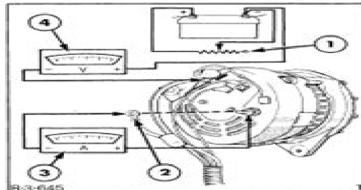
Figure 16 Ground-side Volt Drop Test (Inset showing connection of Millivoltmeter and Variable Load Resistor to Battery)
