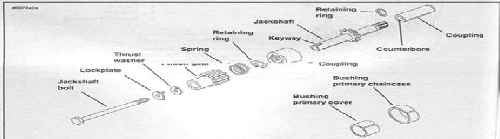
Figure 5-28. Starter Jackshaft
