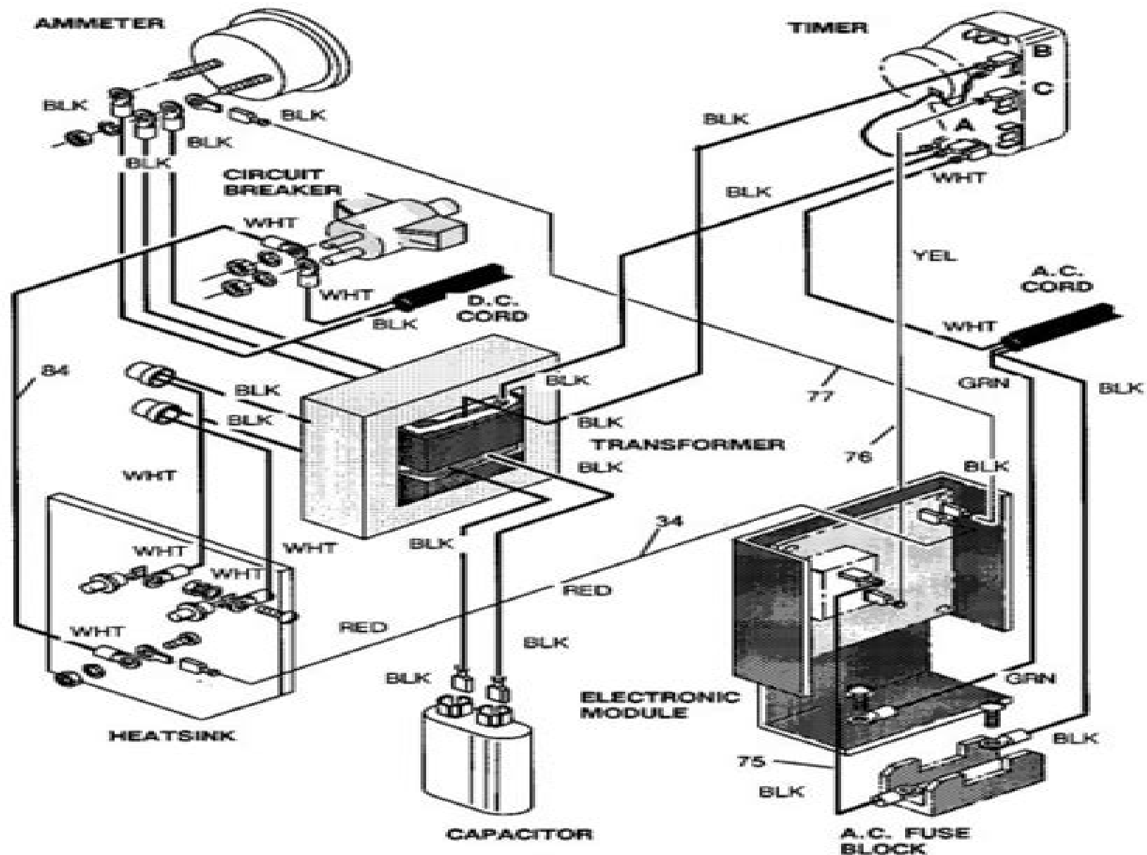
WIRING DIAGRAM (PORTABLE TOTAL CHARGE®)
