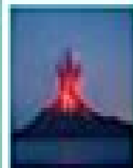
volcanic eruption
