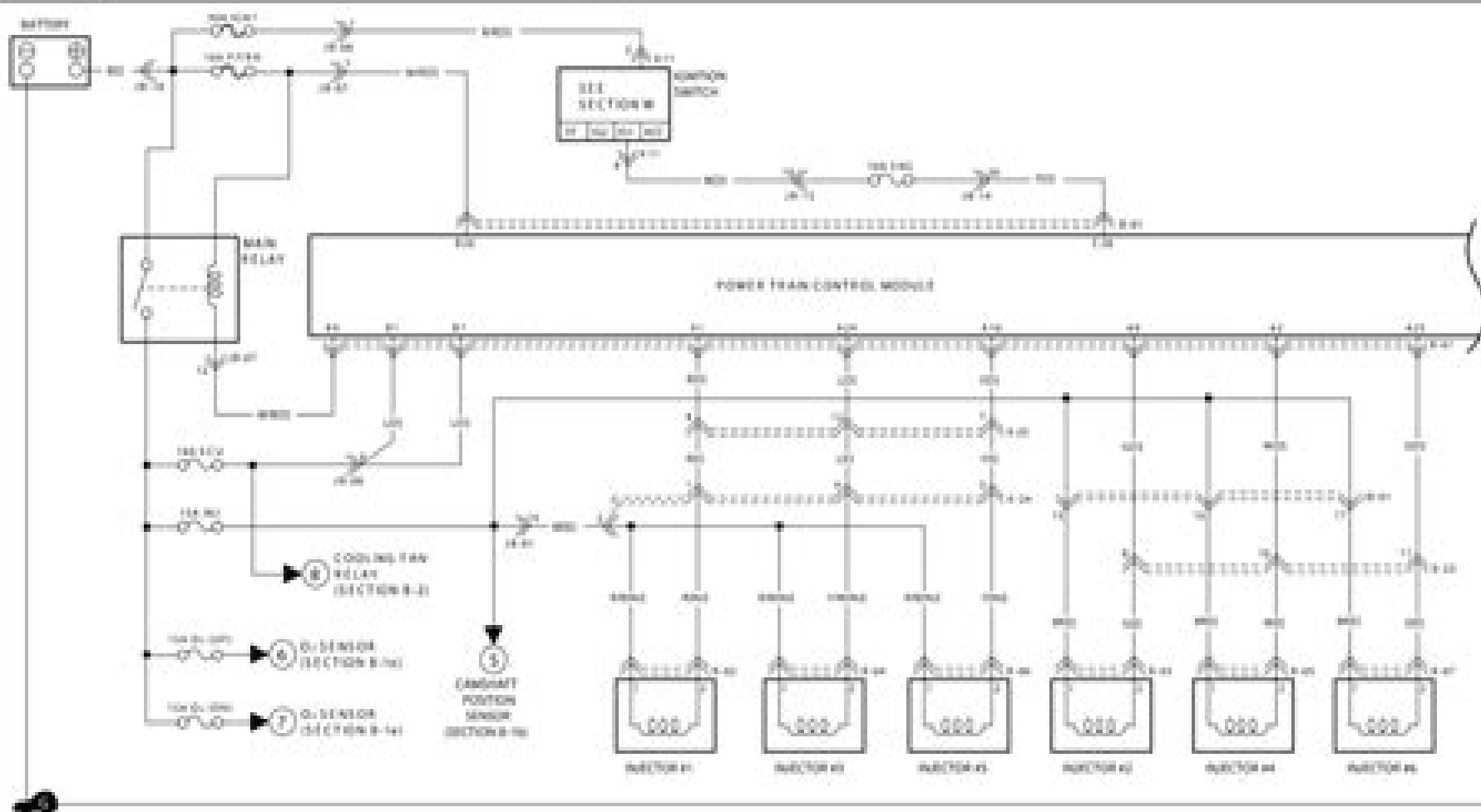
B-1a POWER TRAIN CONTROL, MODULE (2)
