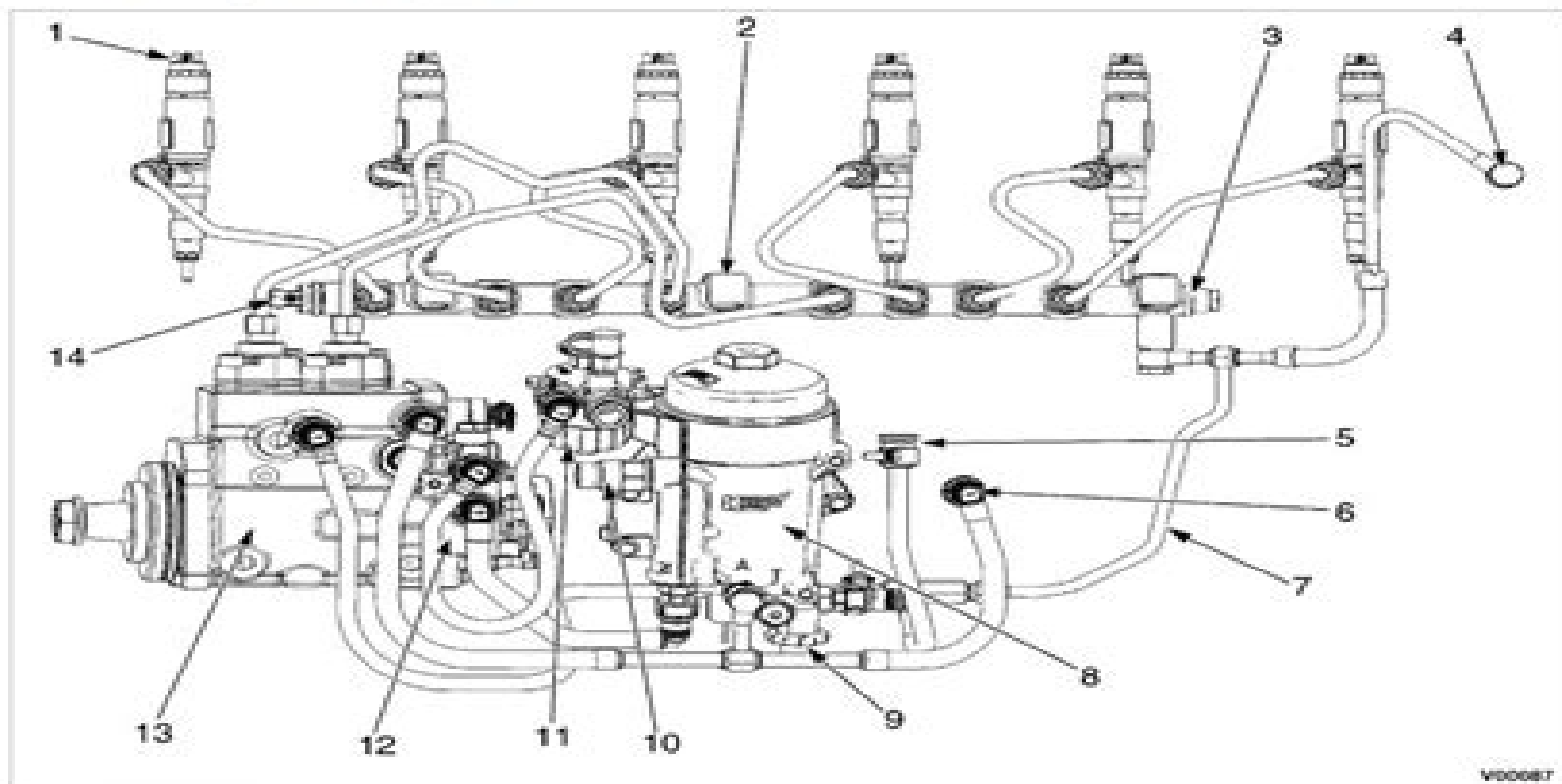
Figure 16 Fuel system
