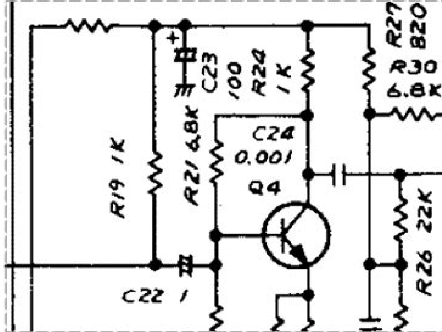
Preview: ICOM IC-25A IC-25E schematic diagram
