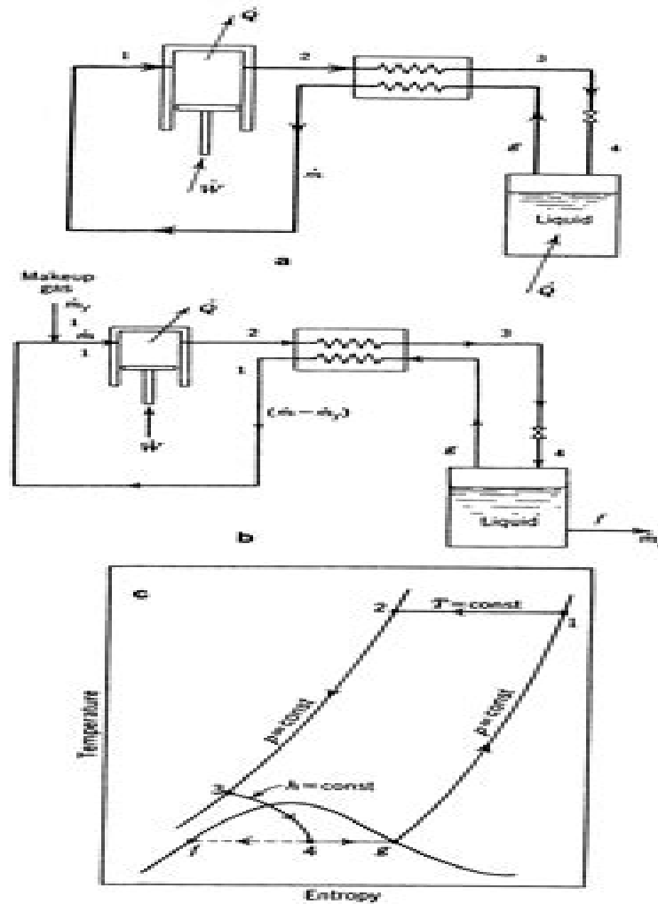
Fig. 4.4. Simple Linde cycle used as (a) a refrigerator or (b) as a Squeefer with (c) the temperature-entropy diagram for both processes.
