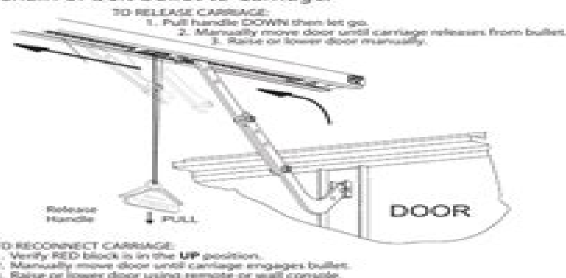
FIG. 6-3 Carriage Release
