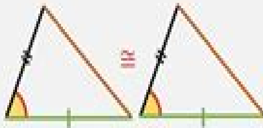
SAS Side-Angle-Side
