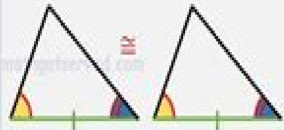
ASA Angle-Side-Angle
