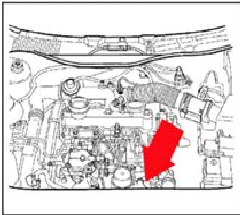
G28 Engine Speed (RPM) sensor (2.0 ltr. engine)
