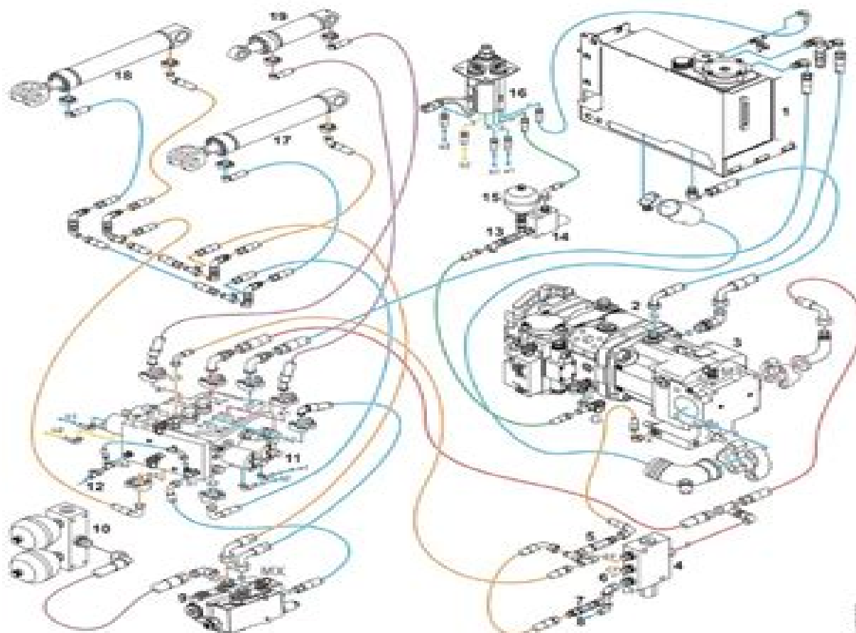
Fig. 250: Main components of the working hydraulics
