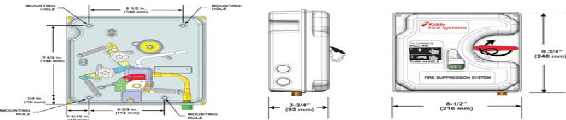
Figure 9. XV Control System Dimensions
