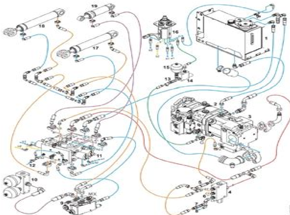
Fig. 250: Main components of the working hydraulics
