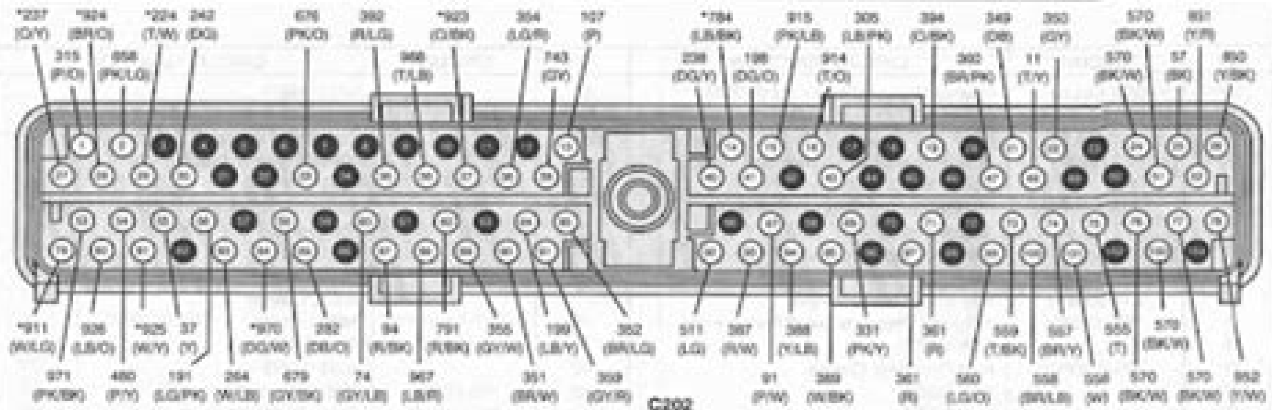
POWERTRAIN CONTROL MODULE (PCM)
