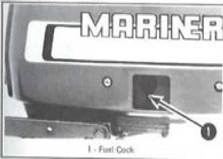
Fig. 8. Fuel Cock (Model 2)
