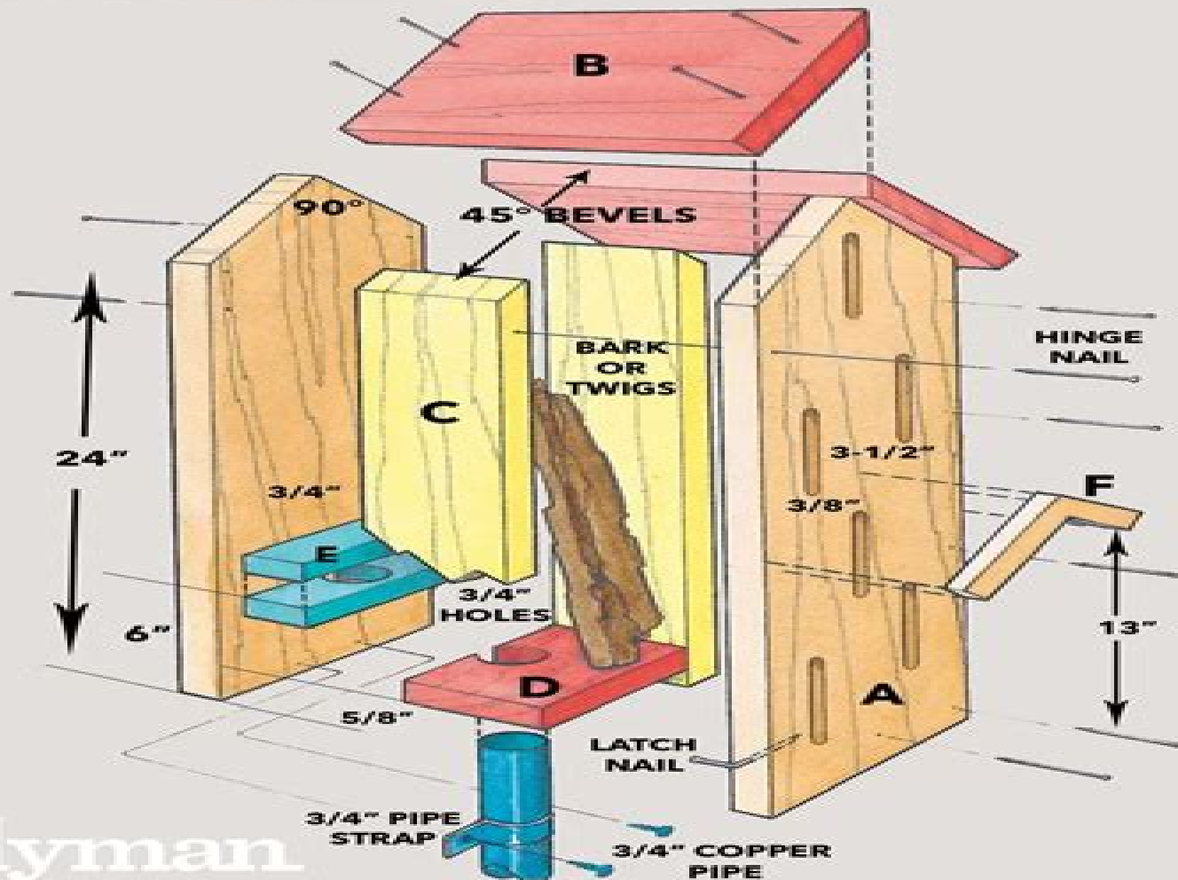
FIGURE A: BUTTERFLY HOUSE
