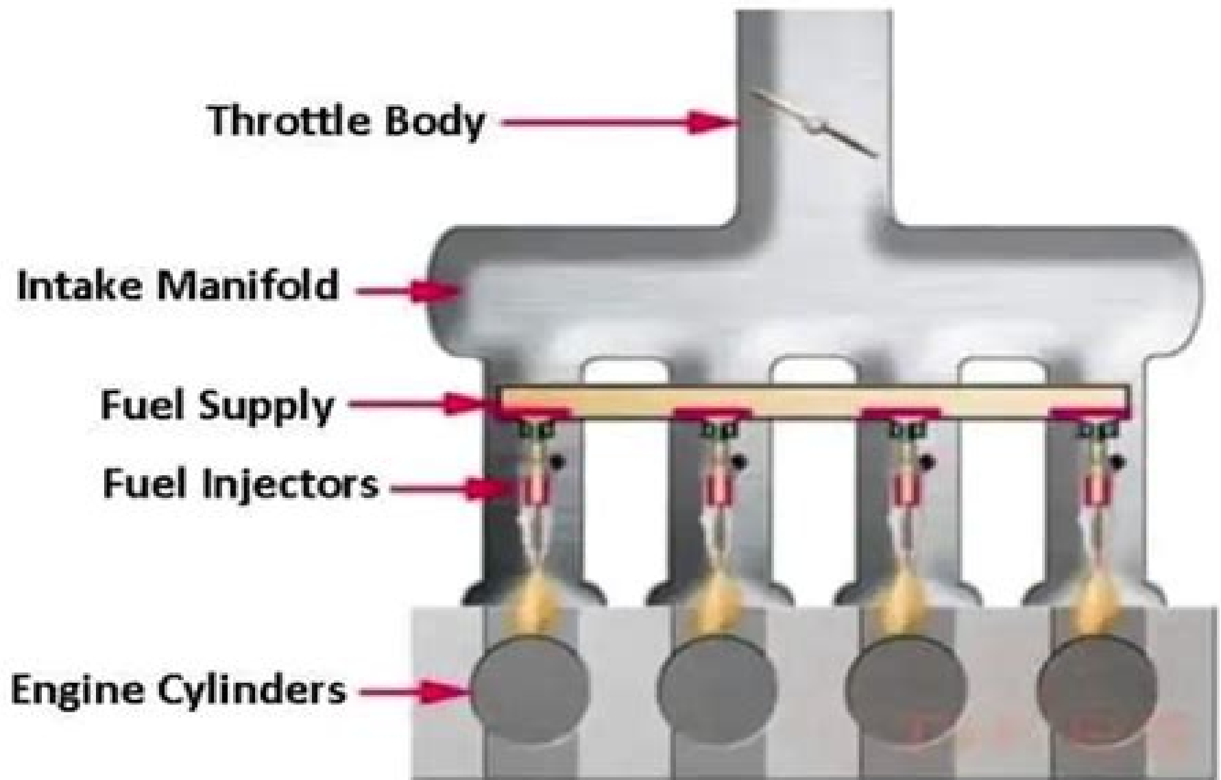
Multi Point Fuel Injection
