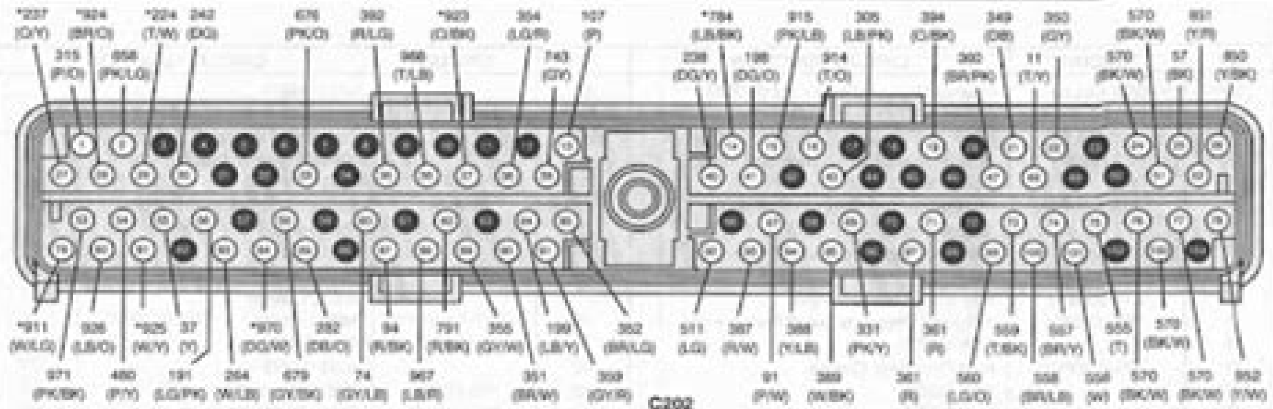
C202 POWERTRAIN CONTROL MODULE (PCM)
