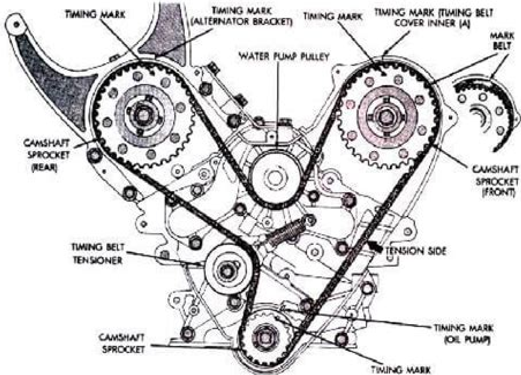
Timing belt alignment marks
