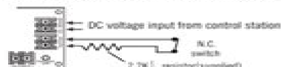
Fig. 2 – Momentary trigger wiring diagram for wet and / or dry N.C. switch.
