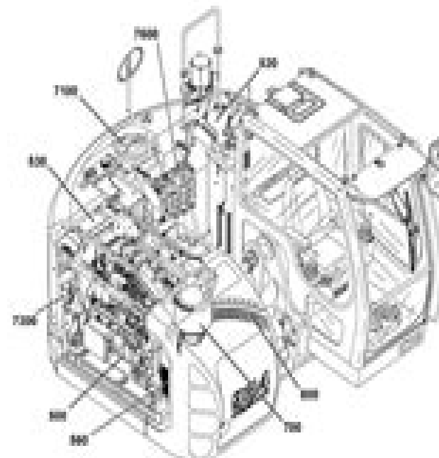
Fig. 1-4 Upper carriage
