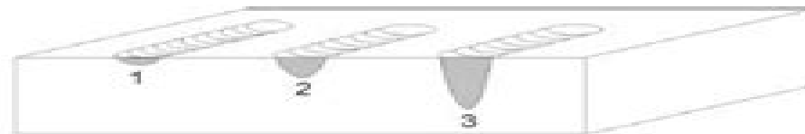
Figure F. Three types of welds created according to the power density and pulse duration of the laser pulse.
