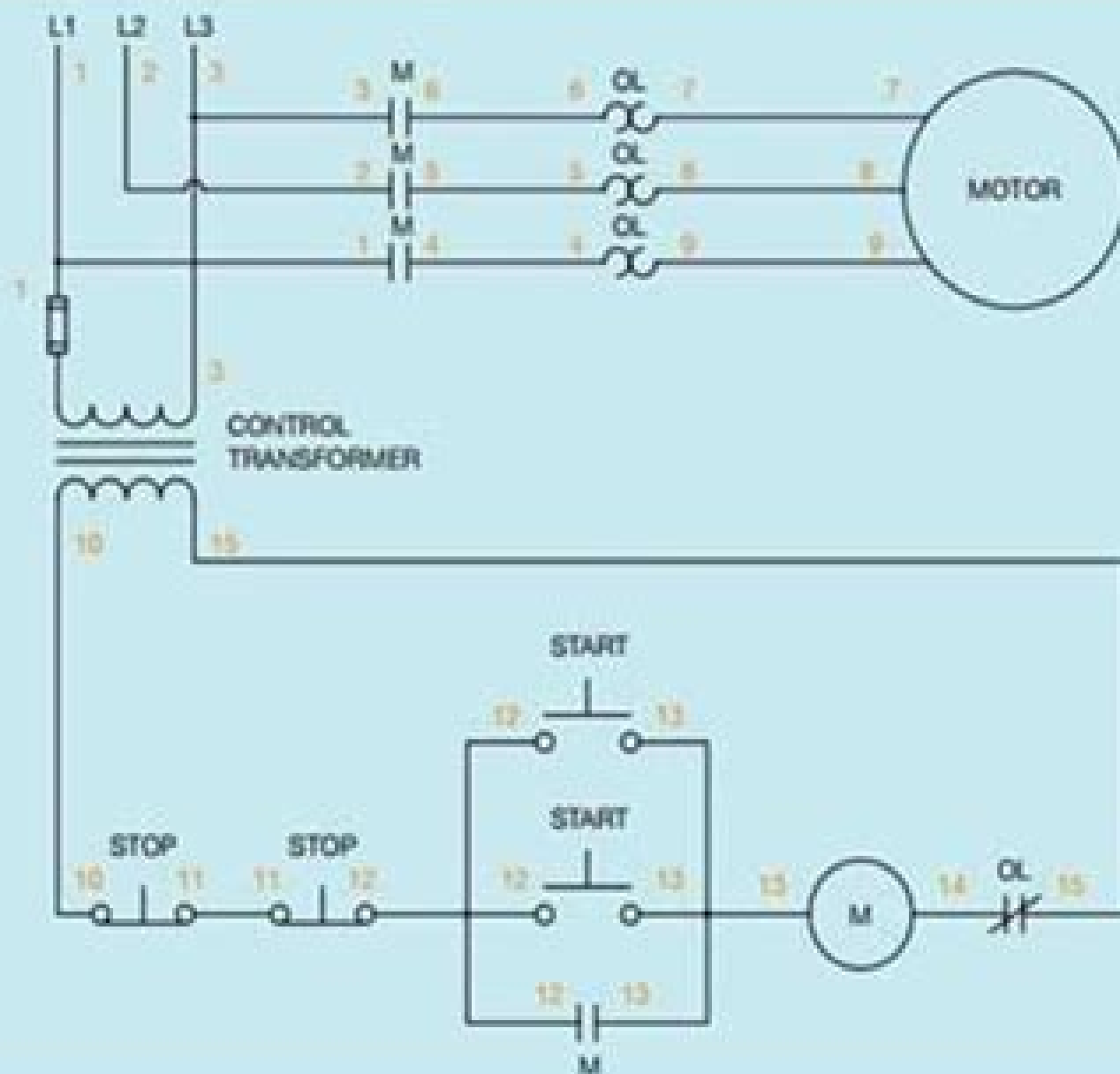
Figure 28-4 Numbers are placed on the schematic. (Source: Delmar/Cengage Learning.)
