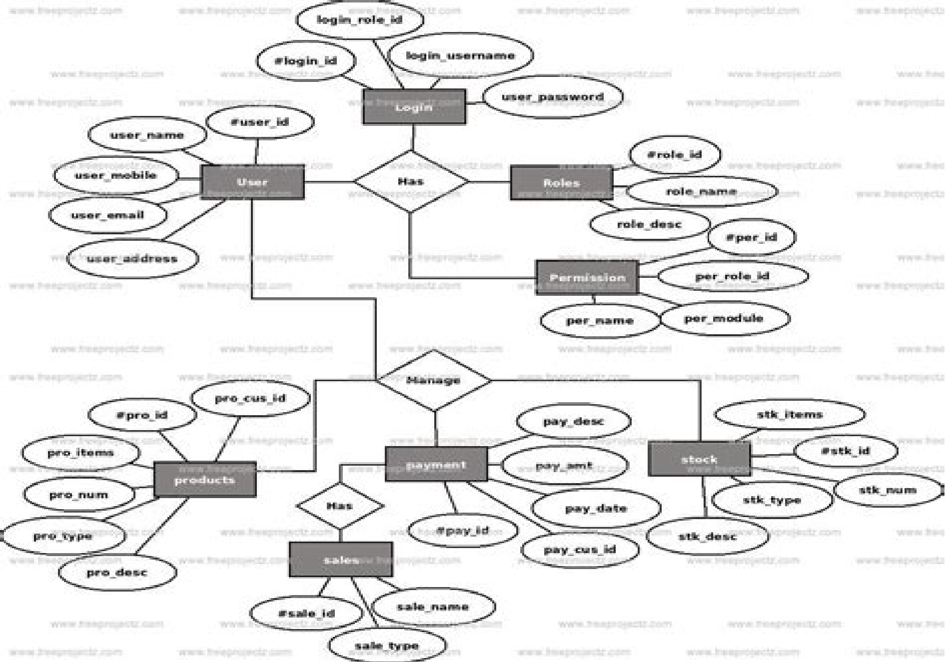
ER Diagram For Department Store Management System
