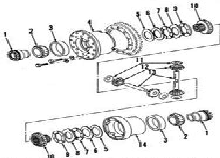
Fig. 282—Exploded view of differential assembly. Note that thick friction disc (9) is installed next to side gear (10) with friction facing towards separator plate (8). Shims (5) are installed between last separator plate and differential case.
