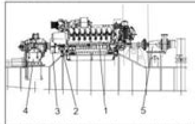
Figure 7.7.6: Direct drive free-standing gearbox arrangement with free and PFI
