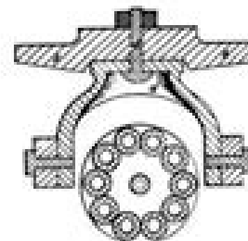
FIG. 5. SECTION THROUGH TRUNION-PLATE TRUNIONS AND PIVOT BLOCK
