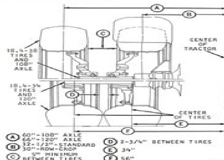
Double Rear Wheel Tread
