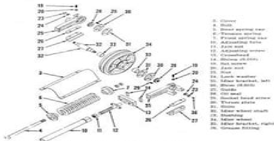
Fig. 42—Exploded view of the front idler assembly used on 4401C and 4401CD tractors.
