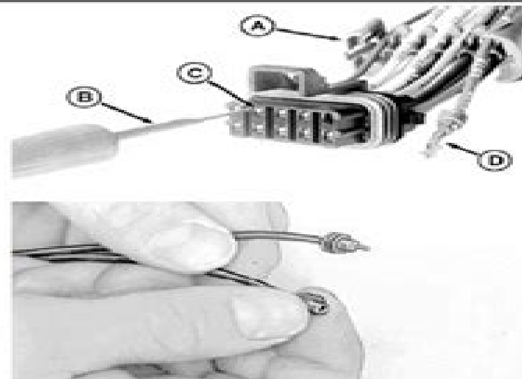
A—Connector Secondary Lock C—Connector Body Socket B—Extraction Tool D—Terminal
